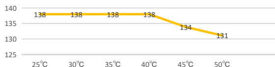
Temperature (Celsius) Derate Curves Unit: kVA
