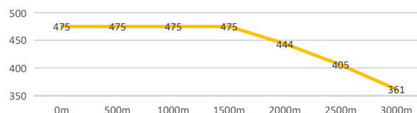
Altitude (meters) Derate Curves Unit: kVA
